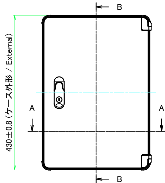
A view
