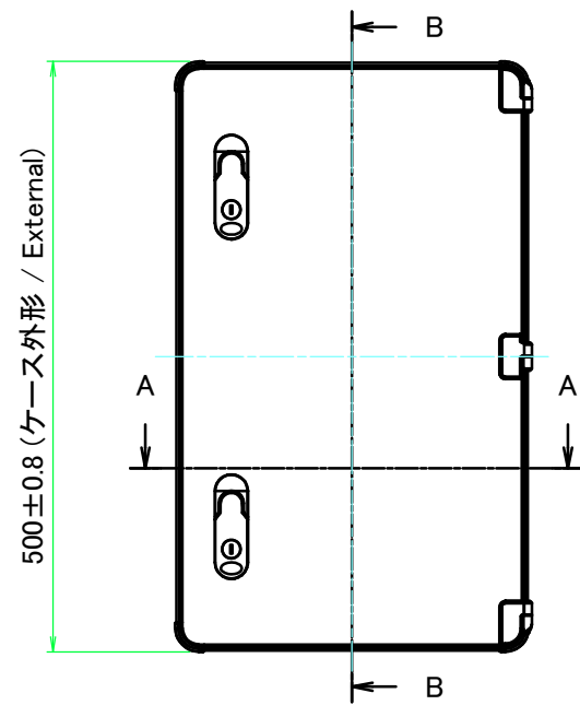
A view
