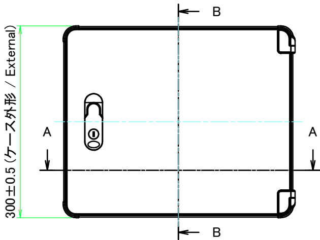
A view
