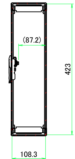
B-B (1:7)
