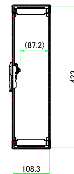
B-B (1:7)
