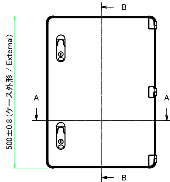
A view
