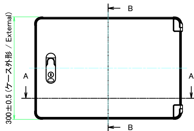
A view
