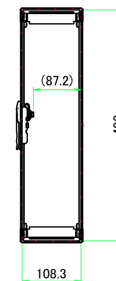
B-B (1:7)
