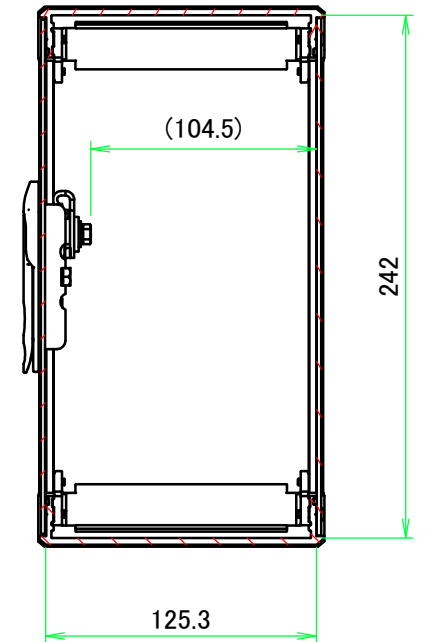
B-B ( 1 :3.5 )
