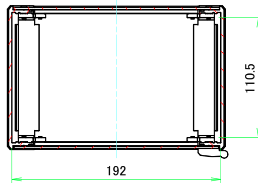
E view
