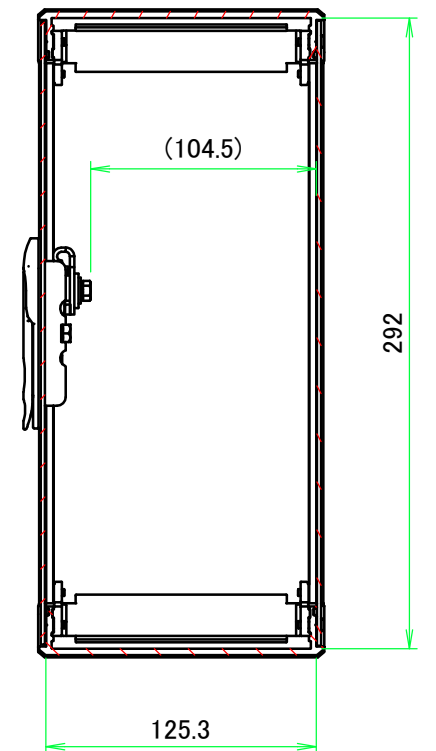
B-B ( 1 :3.5 )
