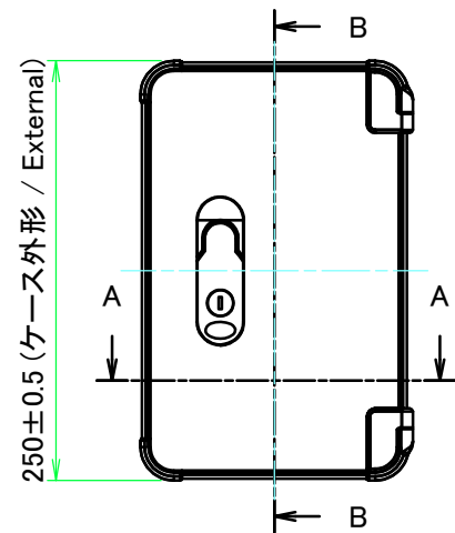
A view
