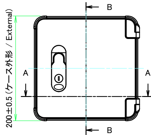
A view
