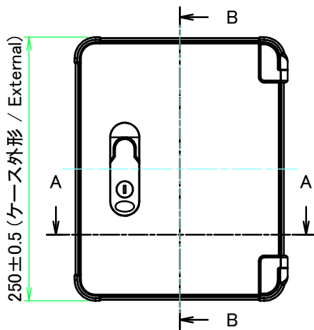
A view
