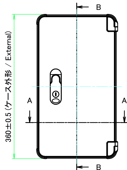
A view
