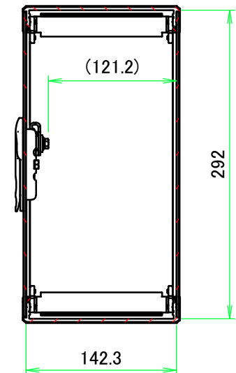
B-B (1:5)
