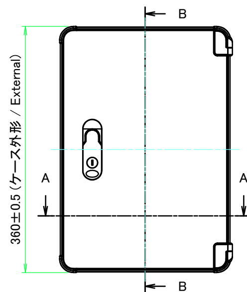
A view
