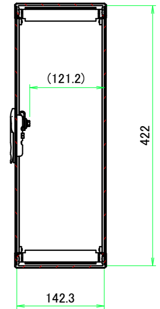
B-B (1:6)
