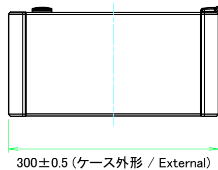
F view
