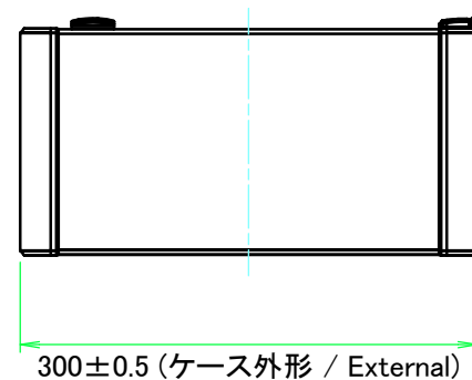
F view
