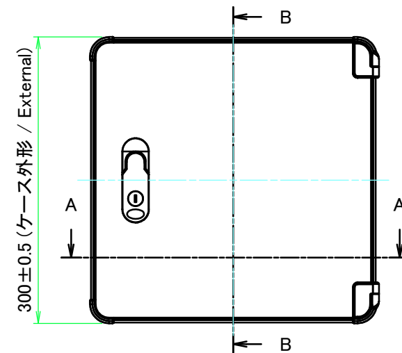
A view
