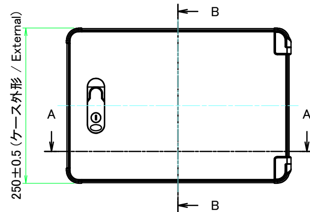
A view
