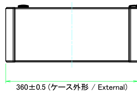
F view
