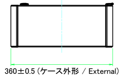
F view
