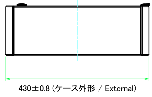
F view
