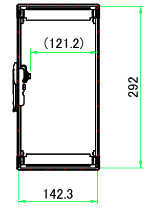
B-B (1:7)
