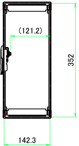
B-B (1:7)
