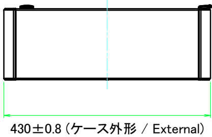
F view
