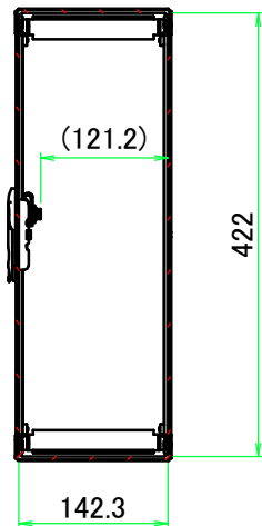
B-B (1:8)
