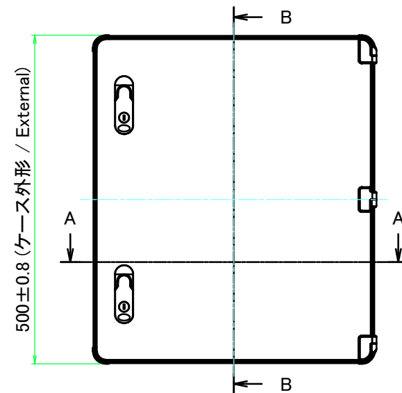
A view
