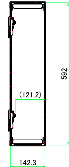
B-B (1:9)
