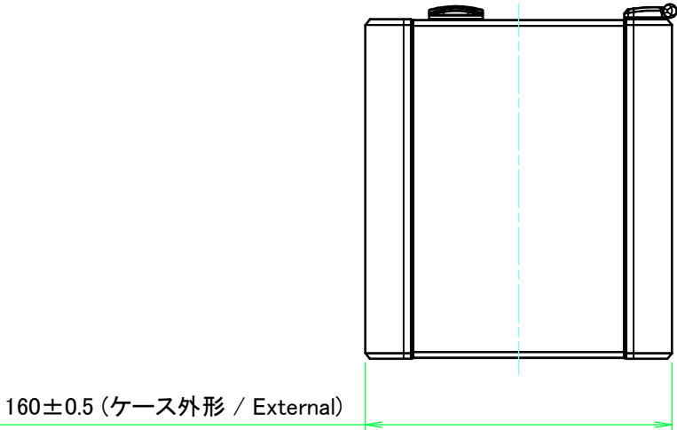
F view
