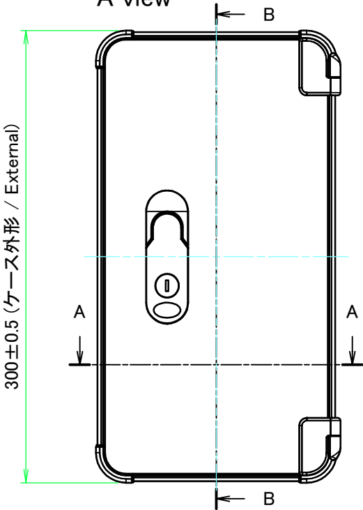
A view
