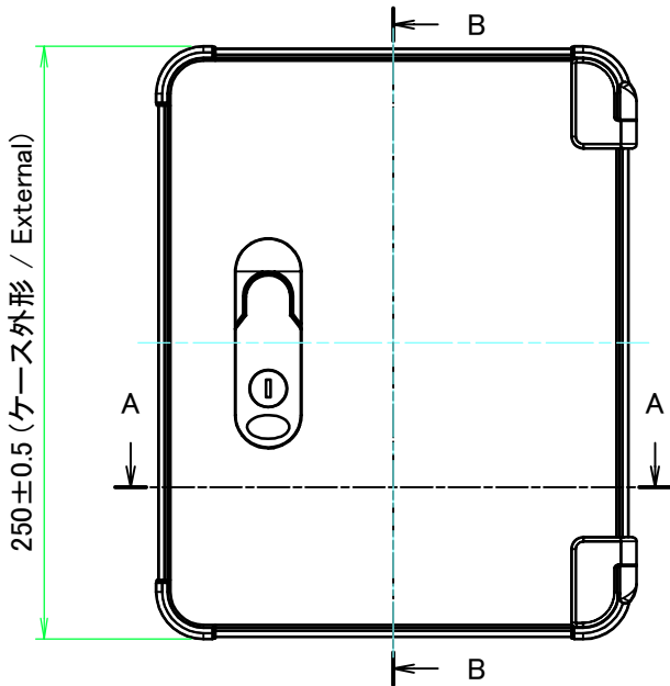
A view
