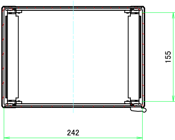
C view
