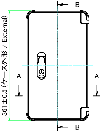
A view
