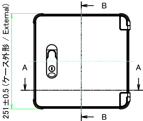
A view
