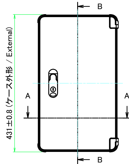
A view
