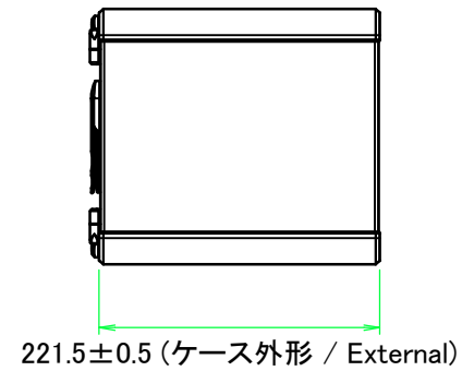
C view
