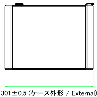
F view
