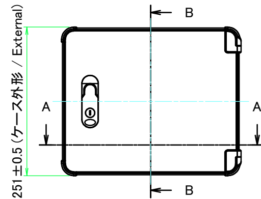
A view
