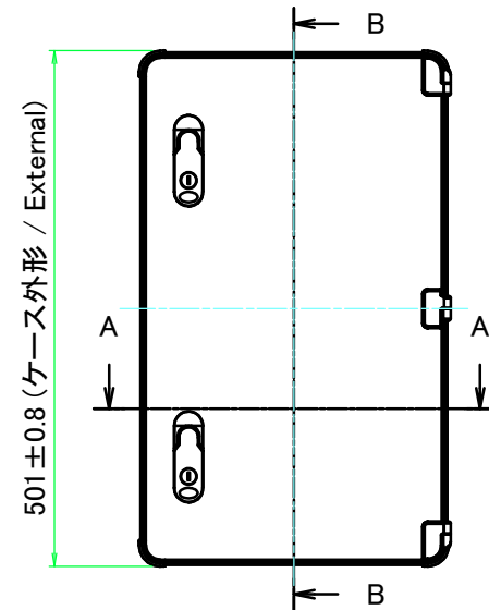
A view
