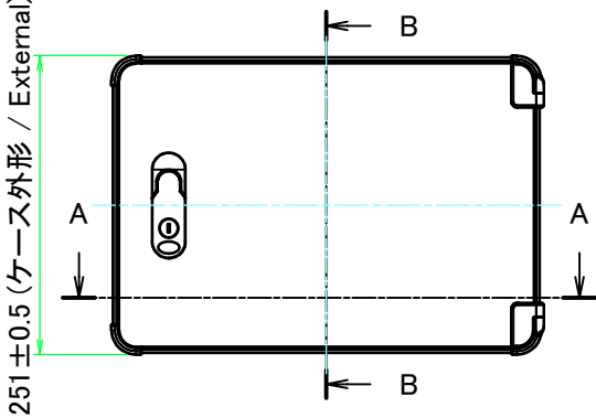
A view
