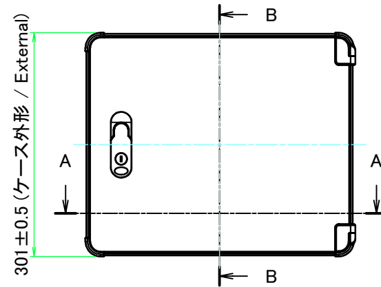
A view
