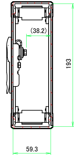
B-B (1:3)
