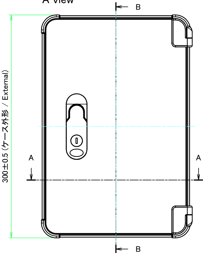
A view
