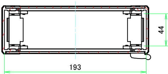
E view
