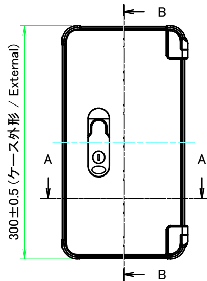
A view
