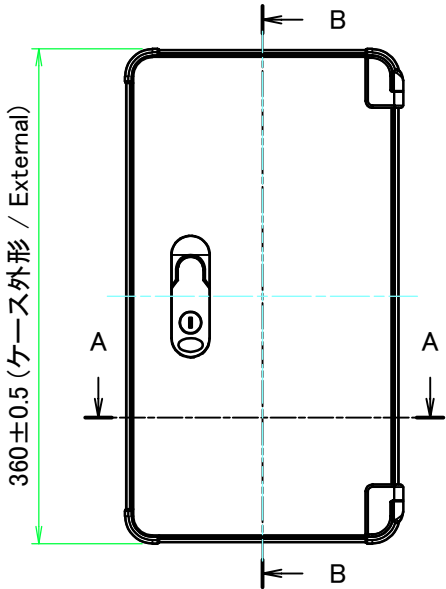
A view
