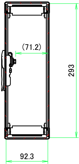
B-B (1:5)
