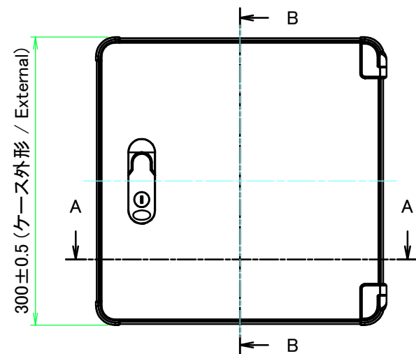
A view
