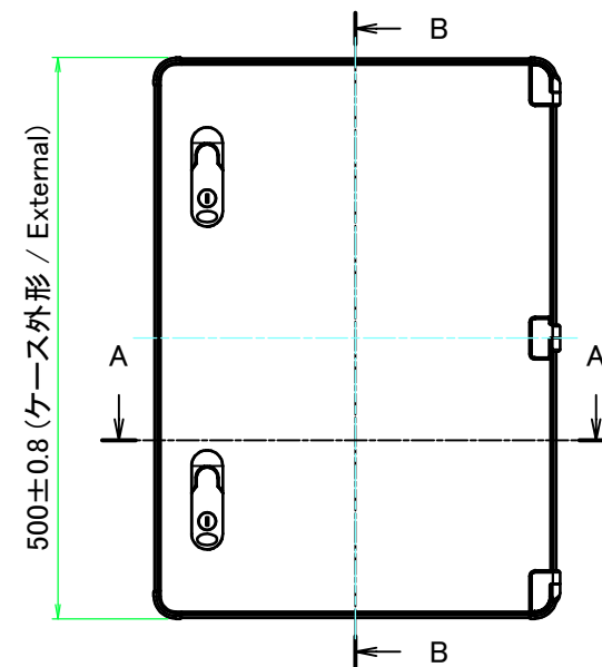
A view
