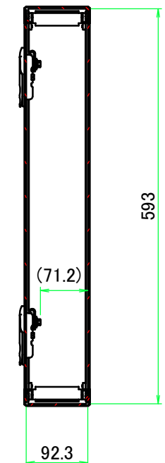
B-B (1:8)
