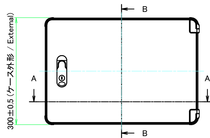
A view
