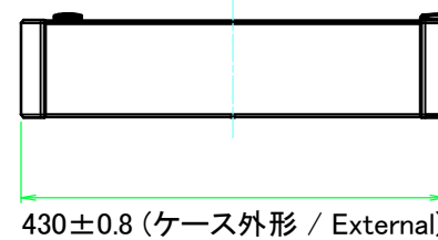
F view
