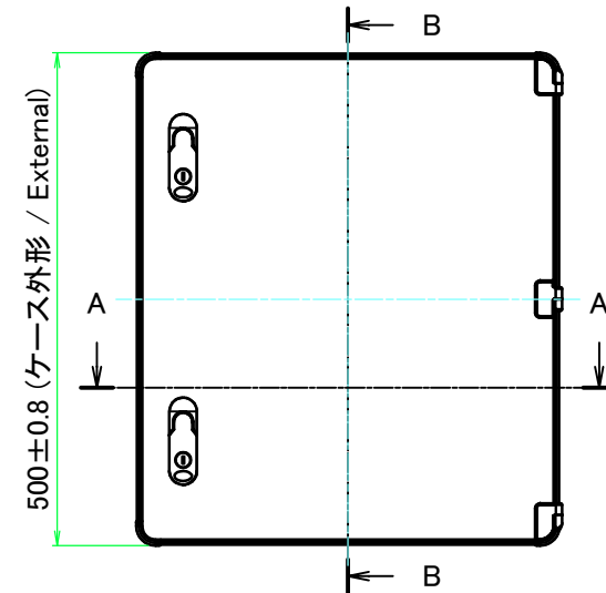
A view
