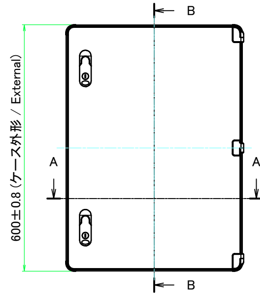
A view
