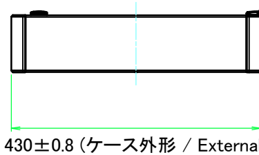
F view
