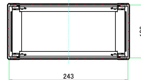
C-C (1:4)
