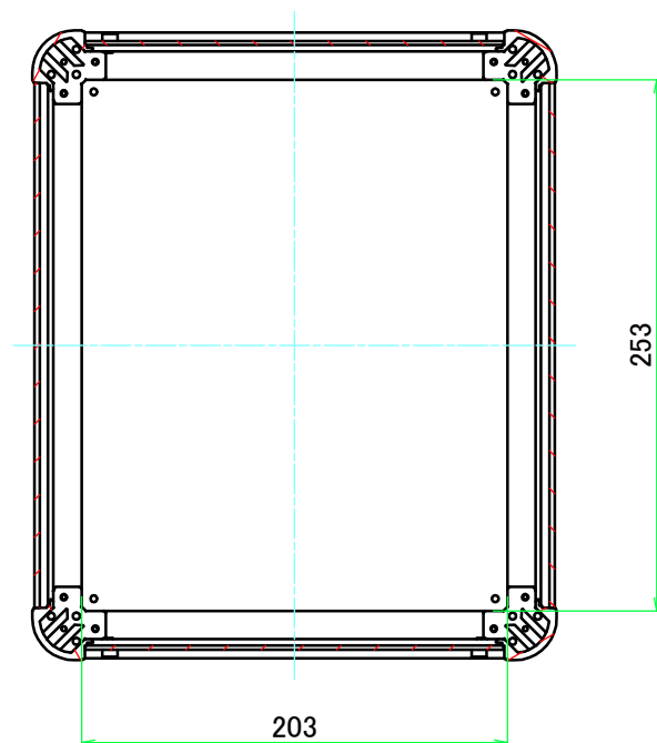
B-B (1:4)
